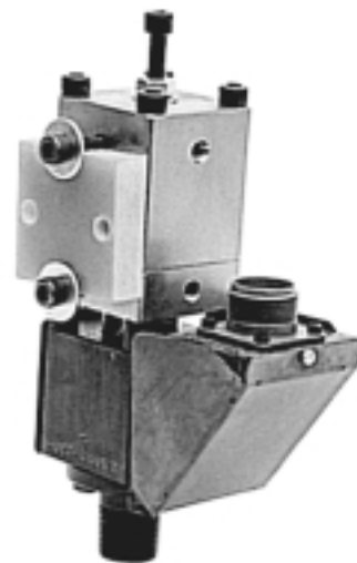
Air-Operated Automatic Hot Melt Dispense Valve (C34079)
