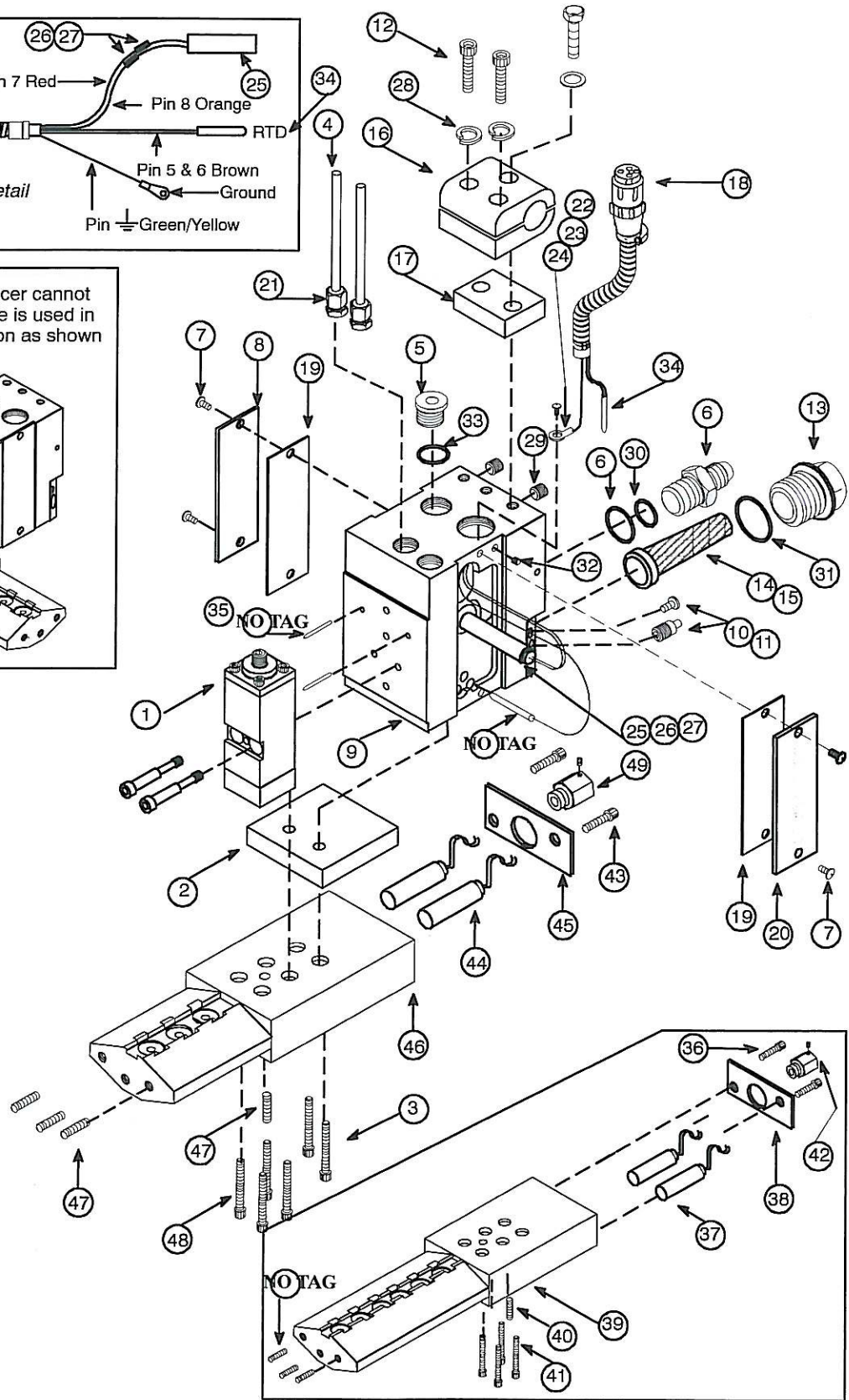
Component Illustration: Head Assembly With Shoe Nozzle
